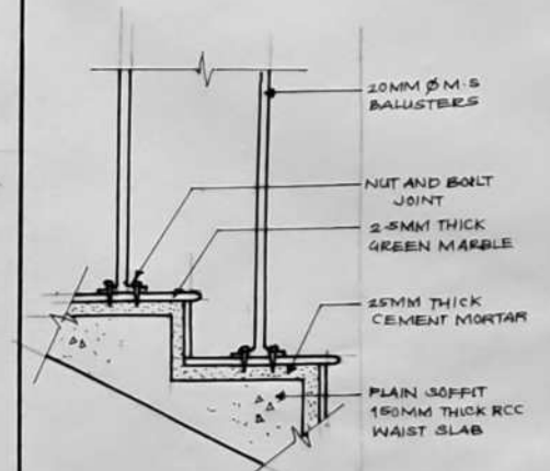
HANDRAIL FIXING DETAIL
