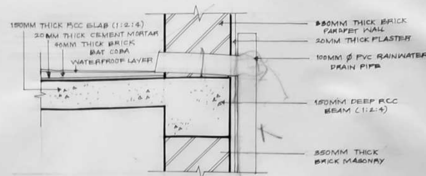
RAIN-WATER DRAIN-PIPE AND COBA DETAIL
