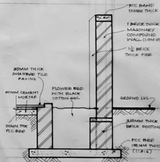
COMPOUND WALL DETAIL SCALE - 1:20
