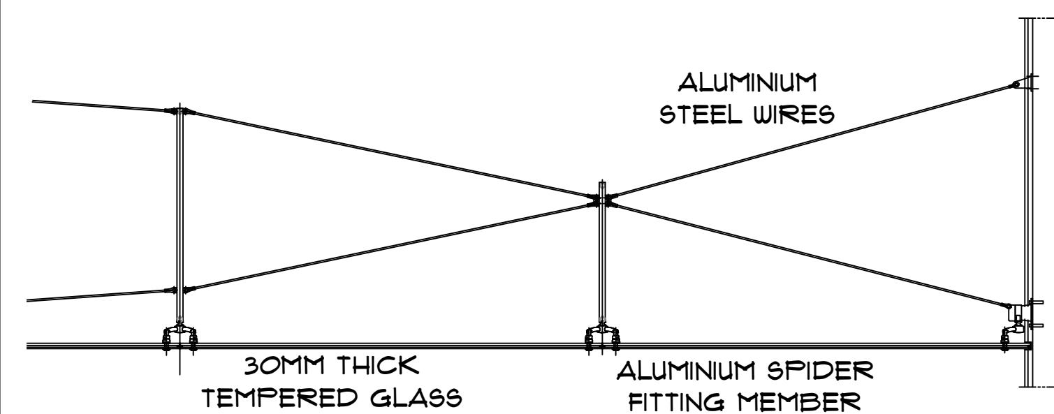
SPIDER FITTING DETAIL IN PLAN SCALE - 1:15
