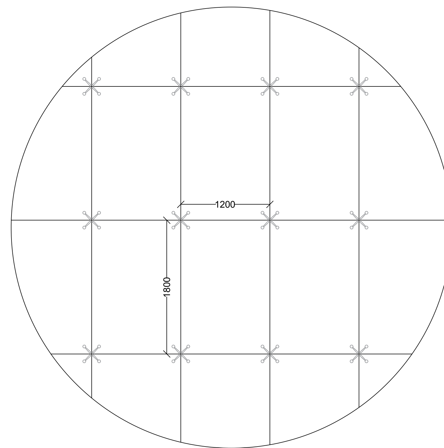
SPIDER FITTING CURTAIN WALL SCALE - 1:30
