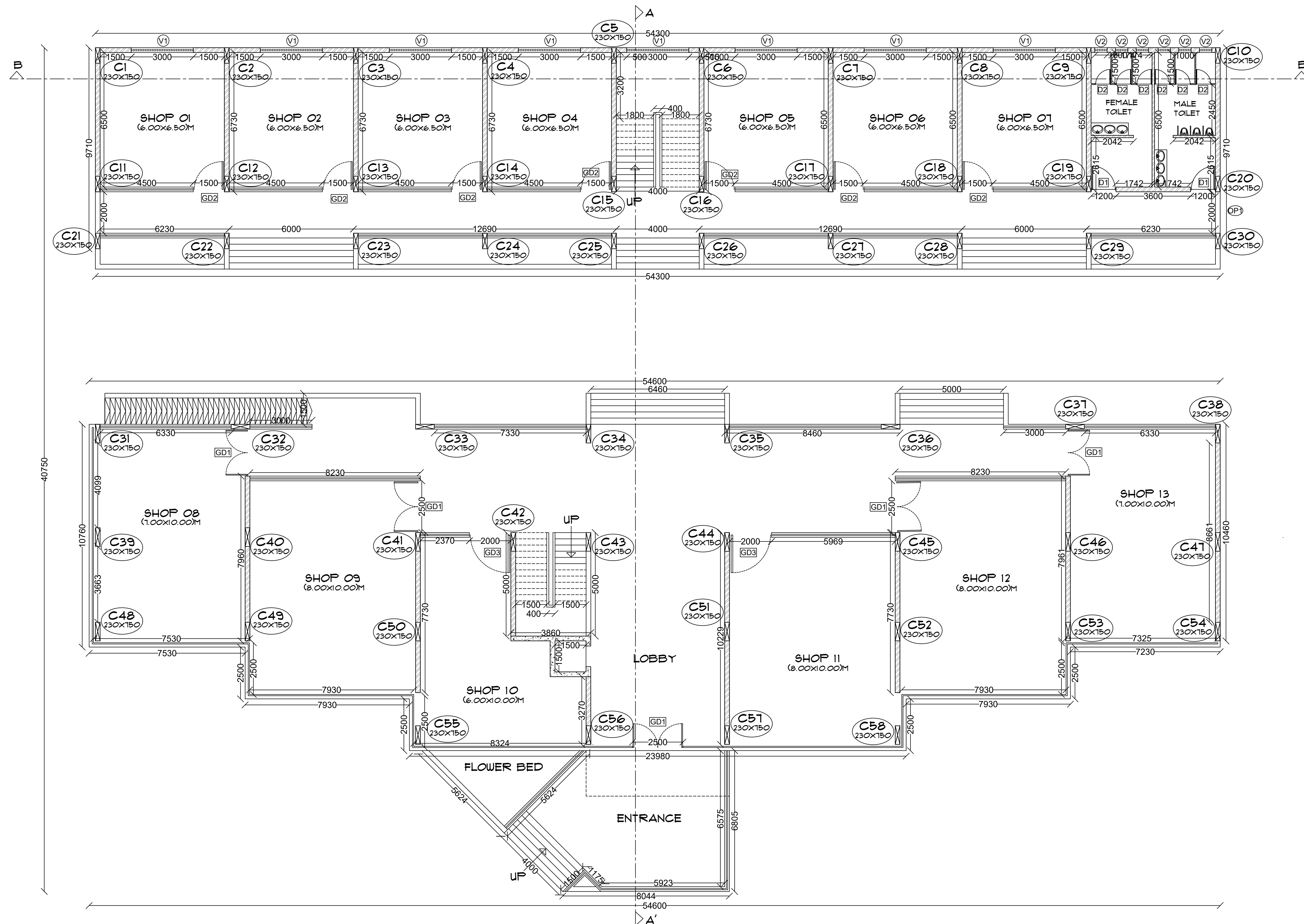
GROUND FOOR PLAN SCALE - 1:100
