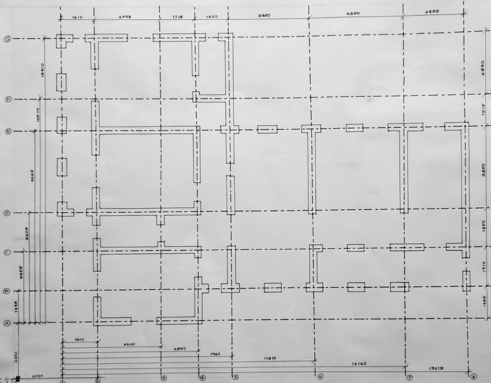
CENTRELINE PLAN
