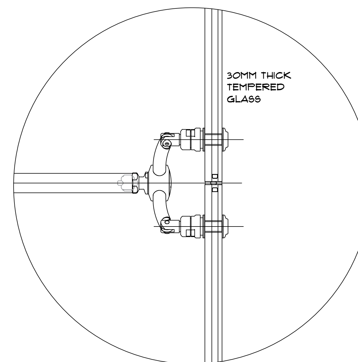
4-WAY FIXING SPIDER FITTING DETAIL SCALE - 1:2
