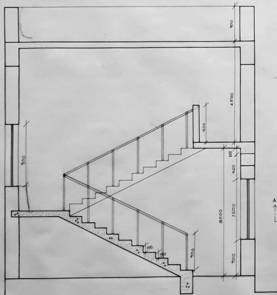
SECTION AA'
