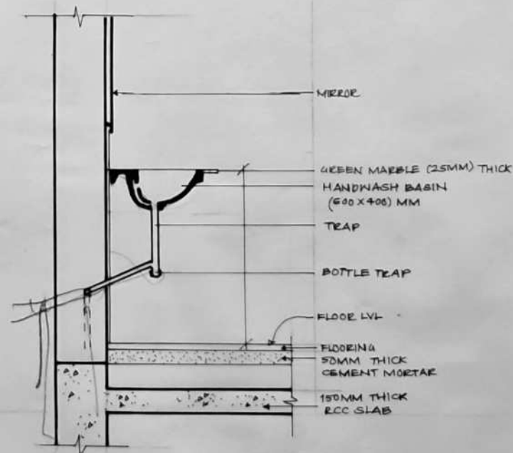
WASH-BASIN DETAIL
