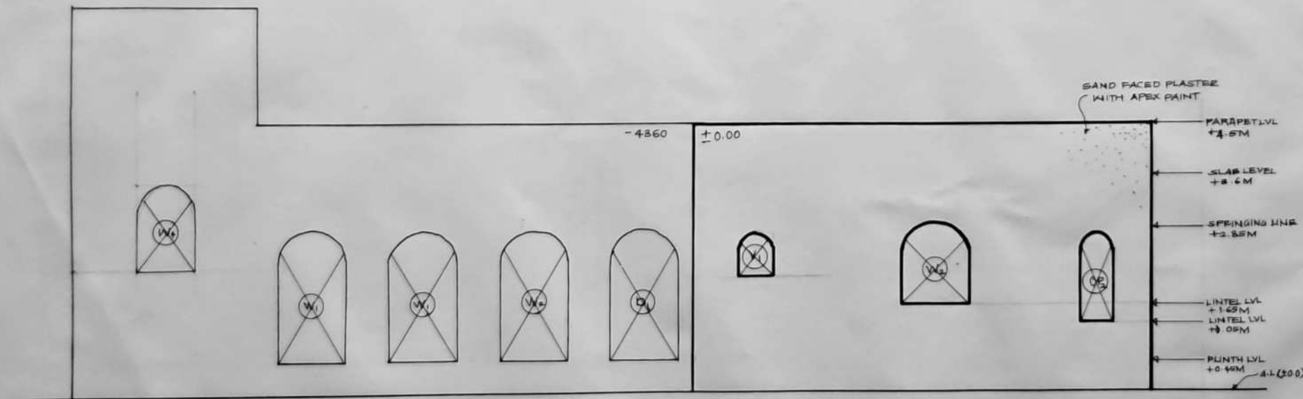
NORTH-SIDE ELEVATION
