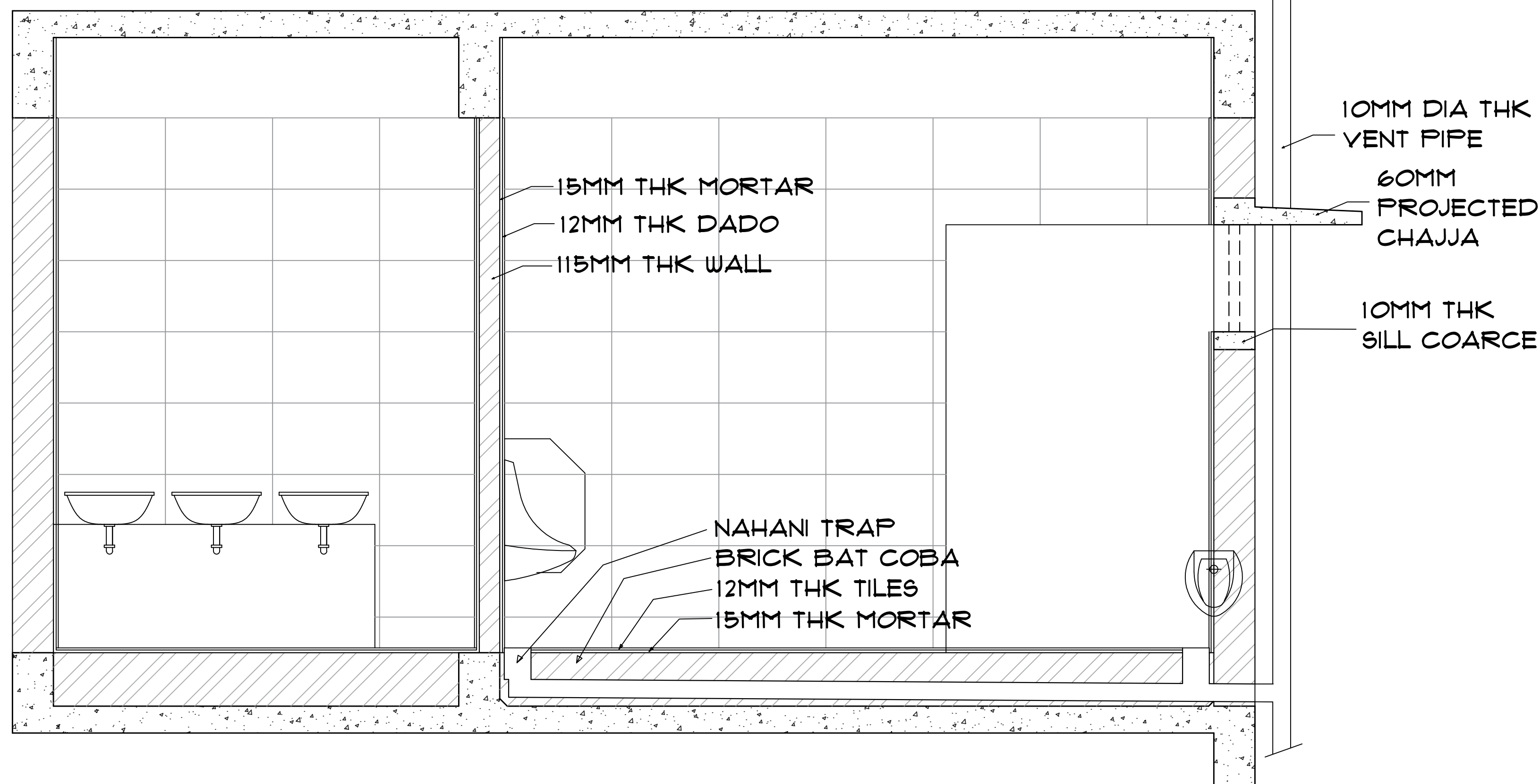
SECTION CC' SCALE - 1:20
