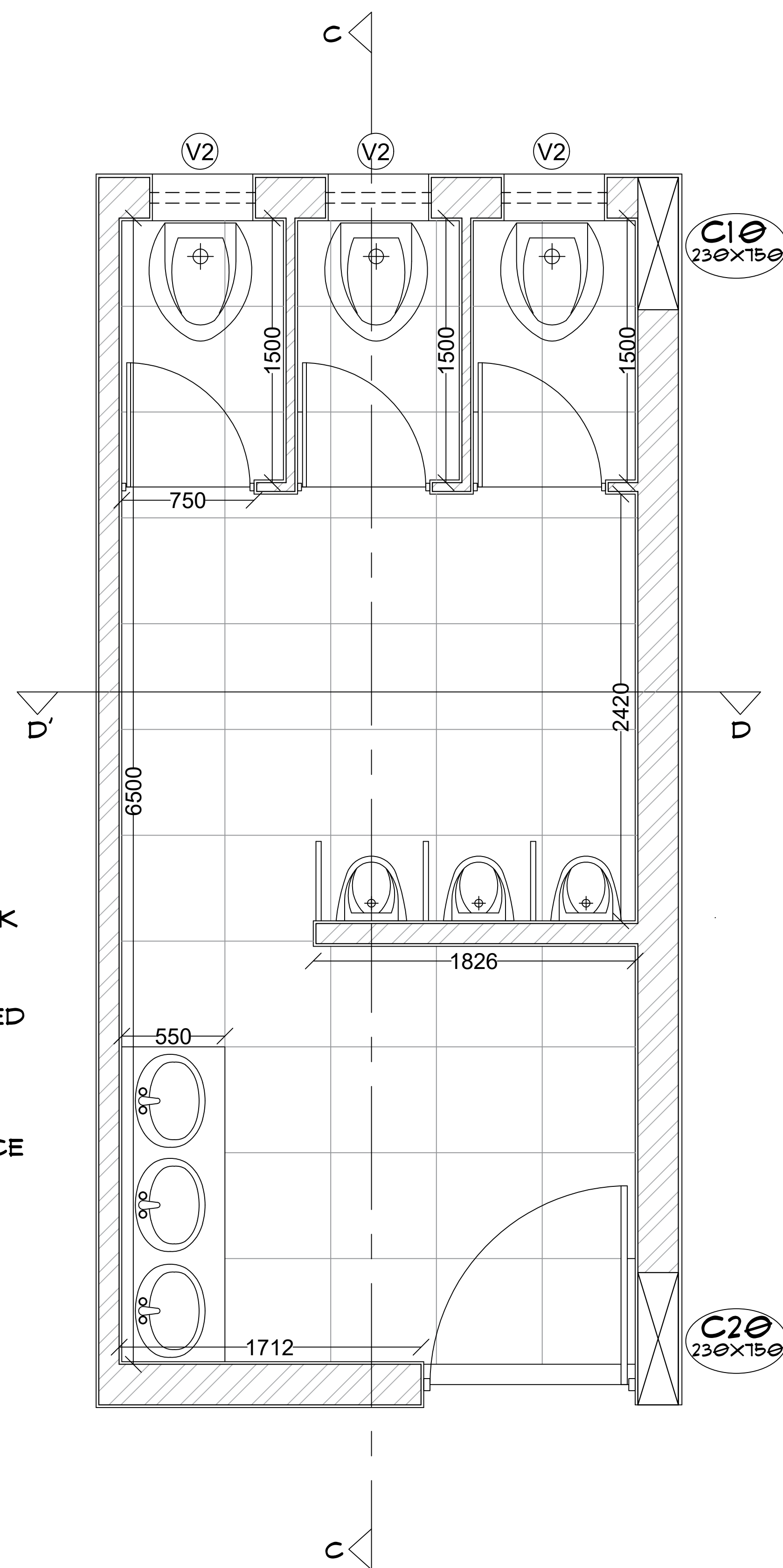
FIRST FLOOR TOILET DETAIL SCALE - 1:20
