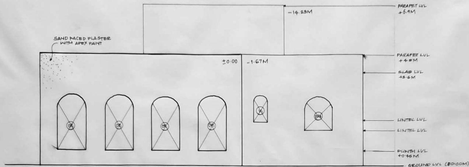
WEST-SIDE ELEVATION
