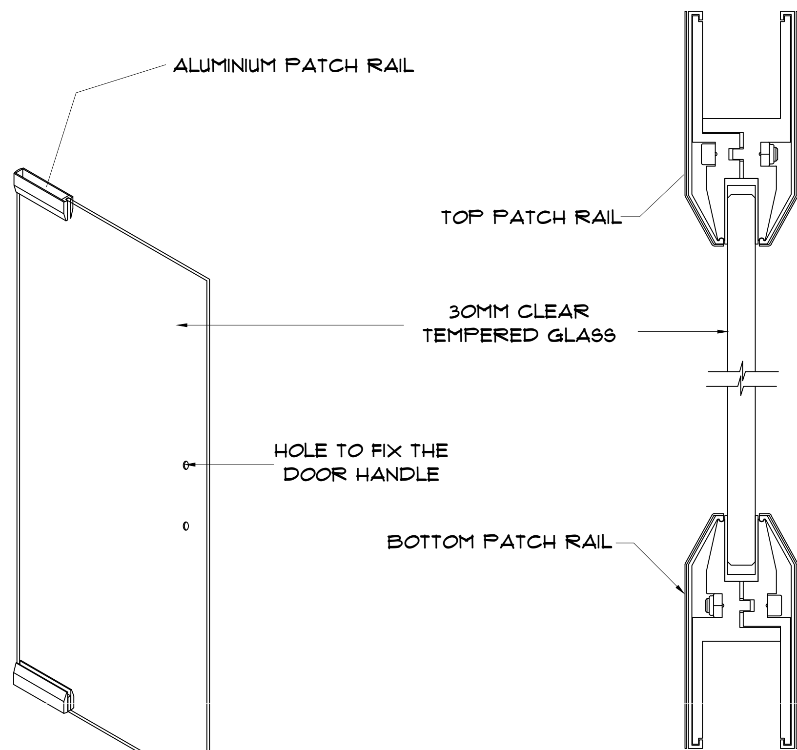
GLASS DOOR WITH ALUMINIUM PATCH RAIL SCALE - 1:4
