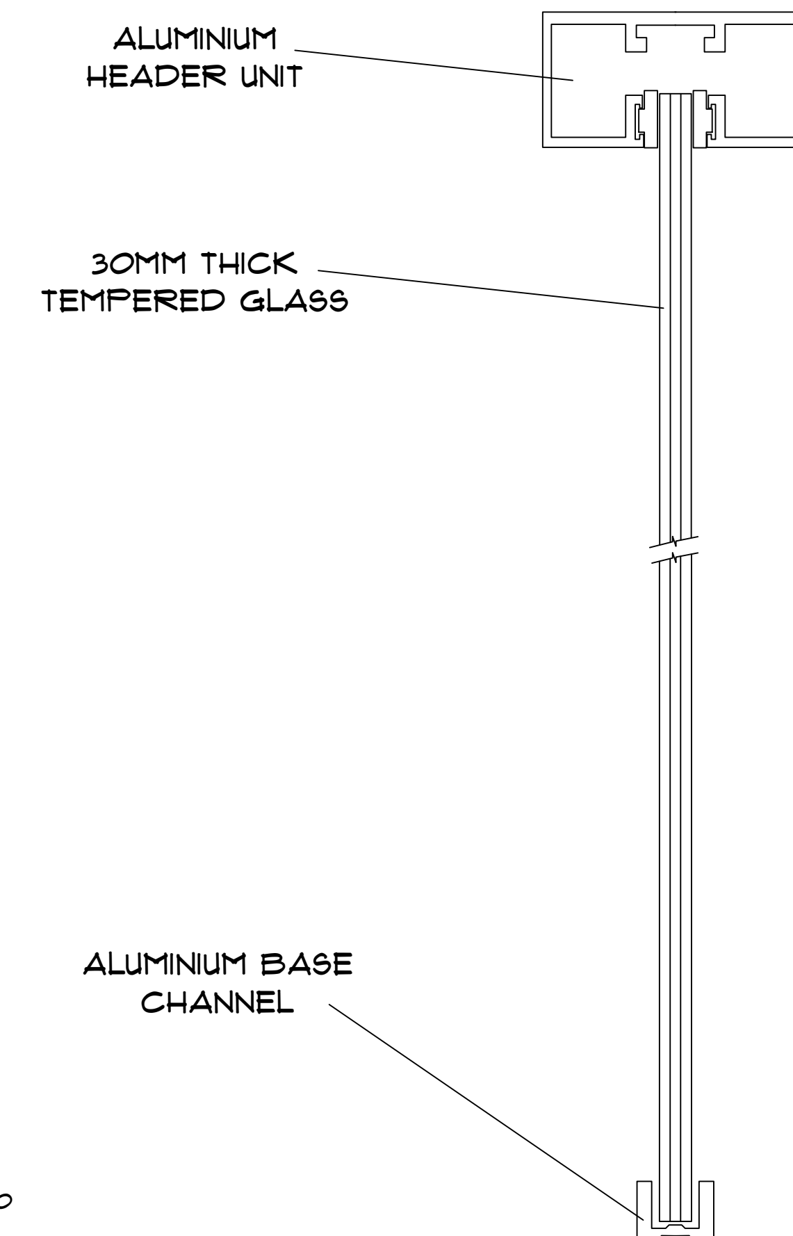
GLASS DOOR WITH ALUMINIUM RAIL SCALE - 1:5
