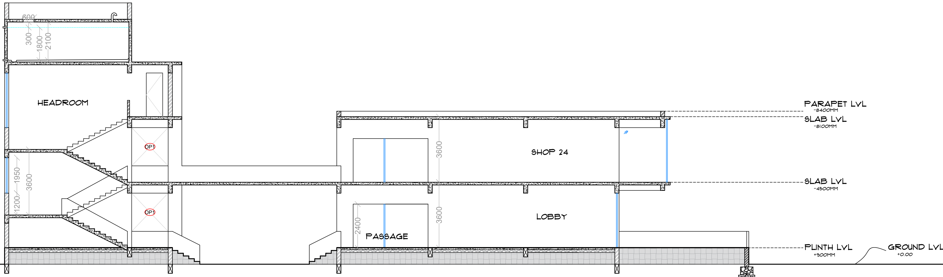
SECTION AA' SCALE - 1:100
