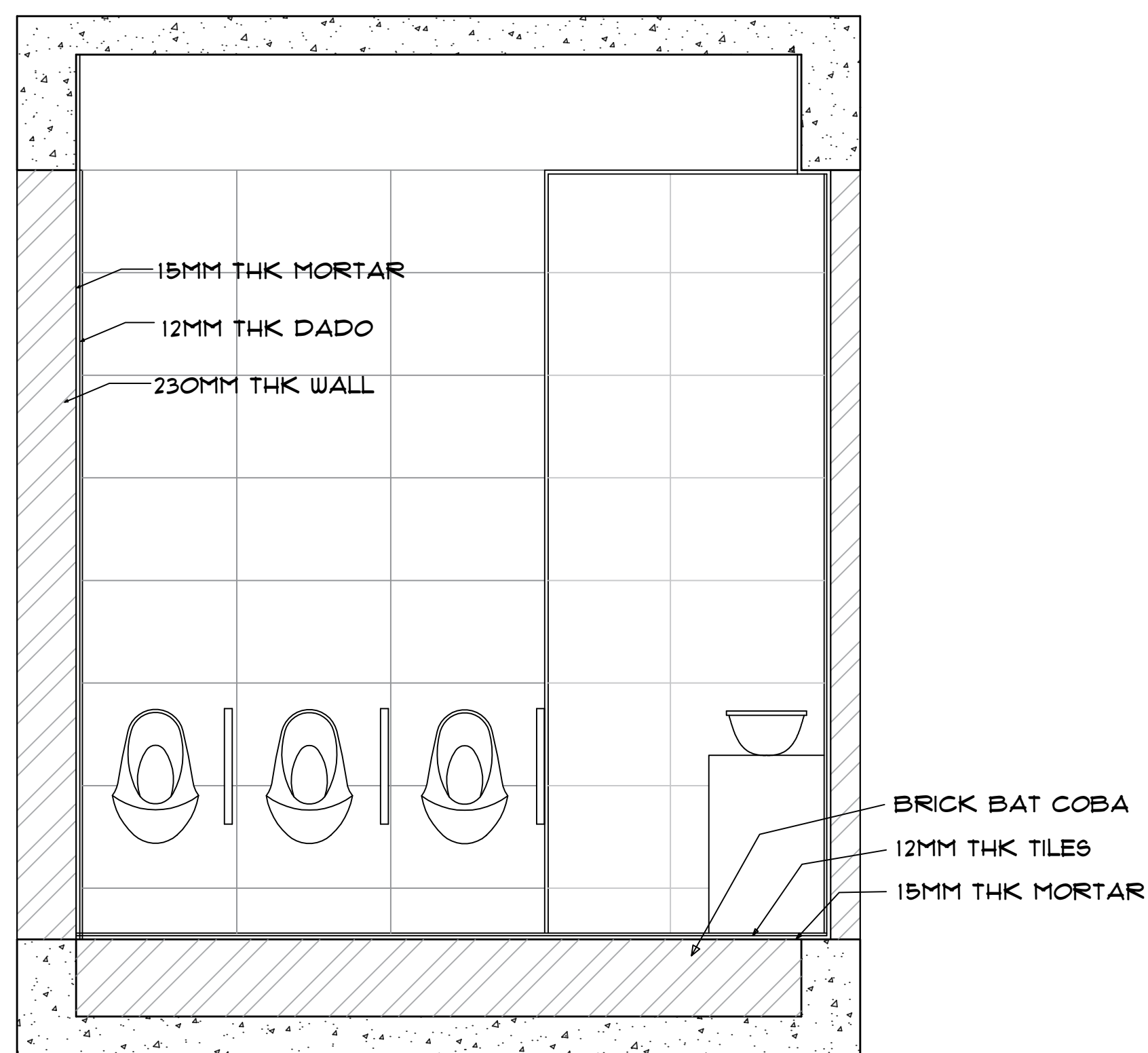
SECTION DD' SCALE - 1:20
