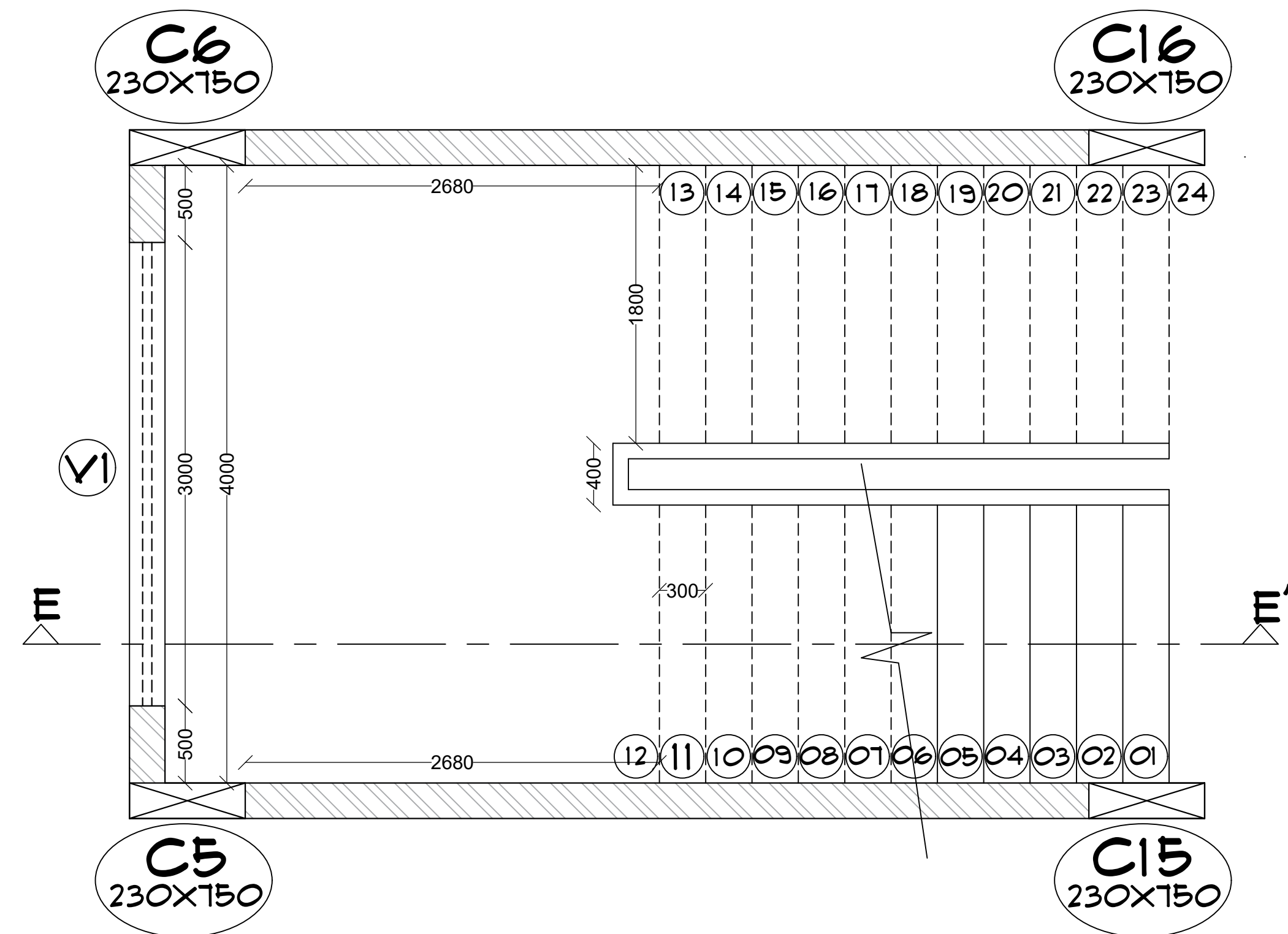
GROUND FLOOR STAIRCASE DETAIL PLAN SCALE - 1:30
