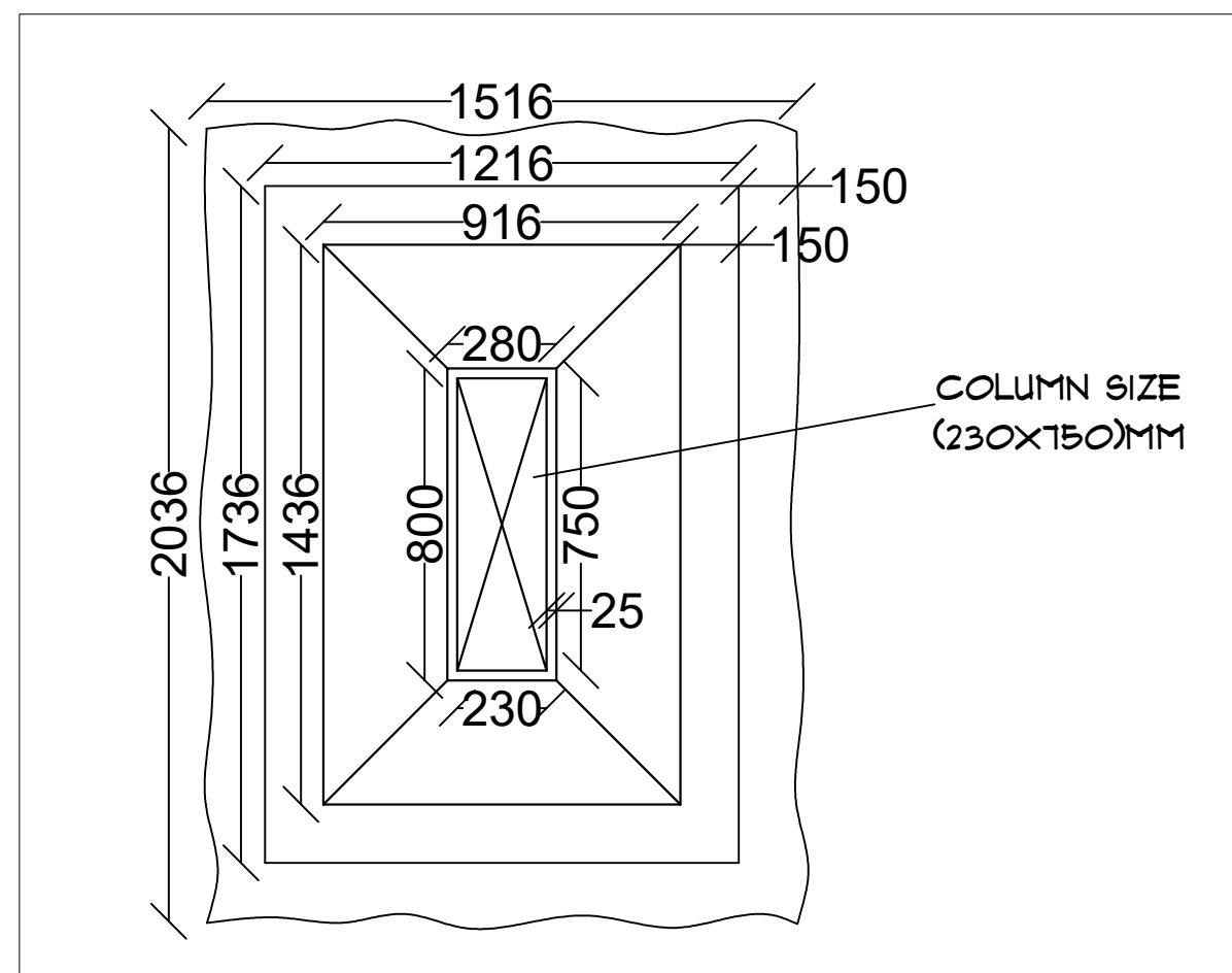
FOUNDATION IN PLAN SCALE - 1:20
