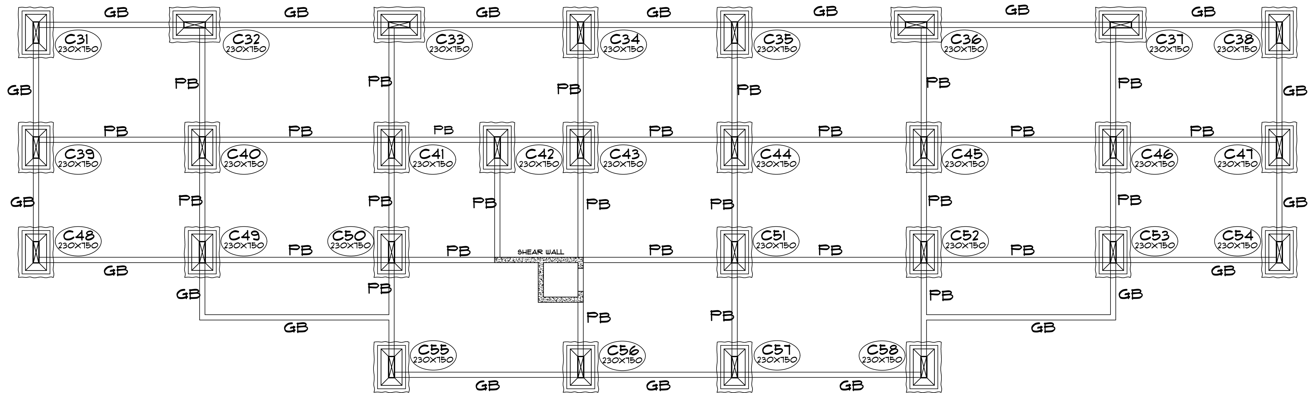
GROUND AND PLINTH BEAM PLAN
