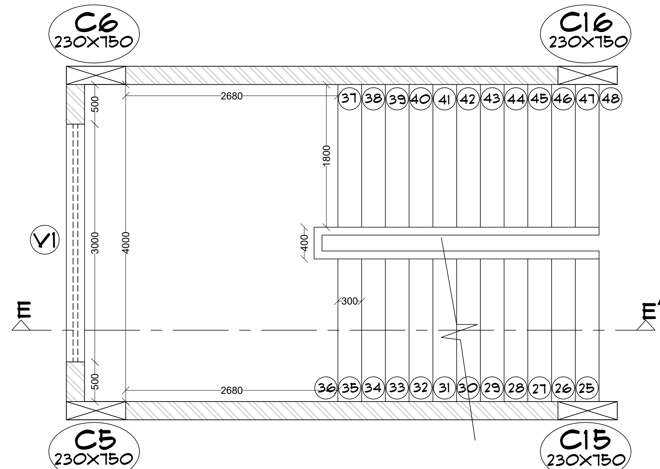
FIRST FLOOR STAIRCASE DETAIL PLAN SCALE - 1:30
