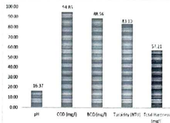
Figure No. 5: Efficiency of Designed Treatment System
