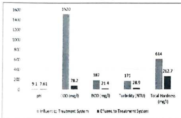
Figure No. 4: Inlet and Outlet Value Designed Filter System
