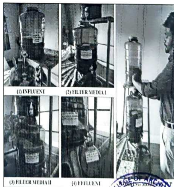
Figure No. 3: Designed and Prepared Light Greywater Treatment System
