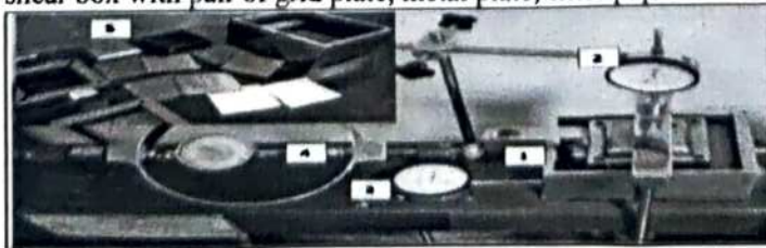
Figure. 2: Experimental set up of direct shear test
